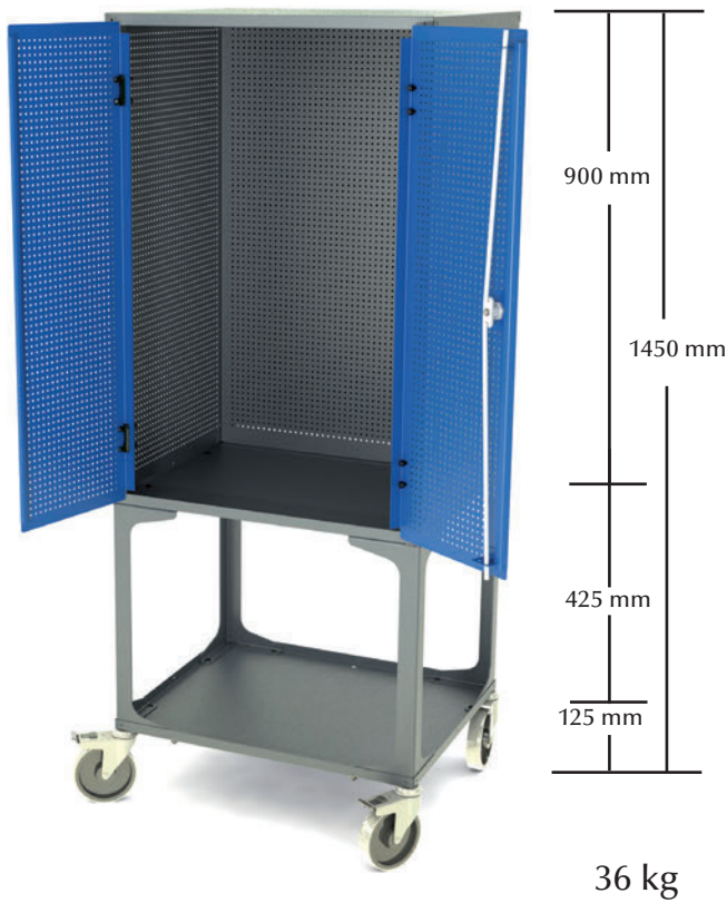
UPPLAGSVAGN STOCK TROLLEY Article no. 800080
